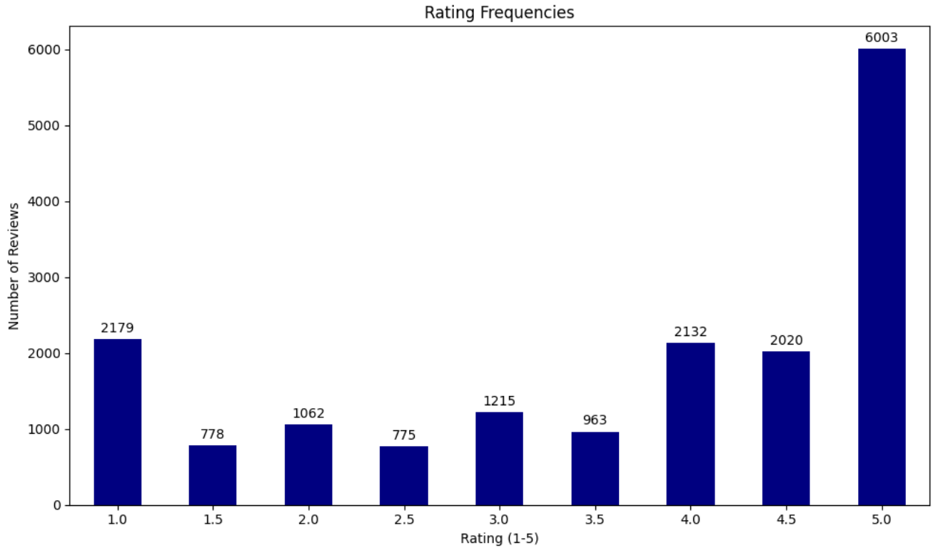
Figure 2. Rating frequencies.
